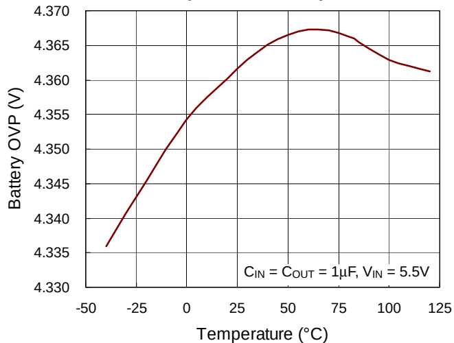
Battery OVP vs. Temperature
