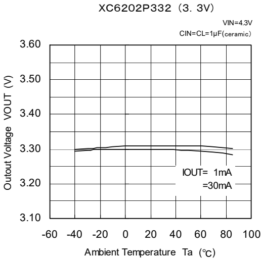
(5) Output Voltage vs. Ambient Temperature
