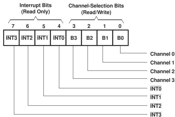
Figure 8-8. Control Register
